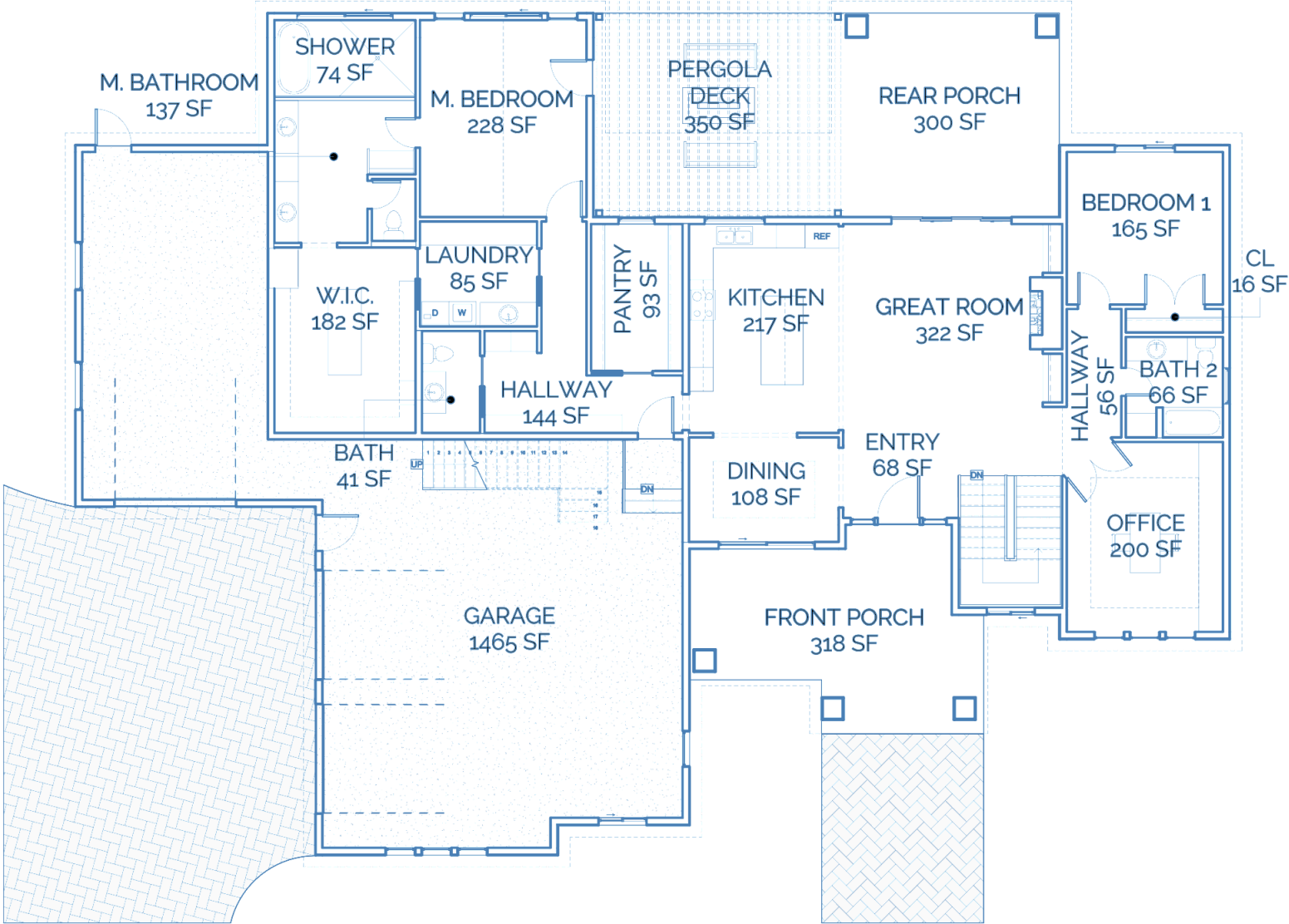
First floor NTS
