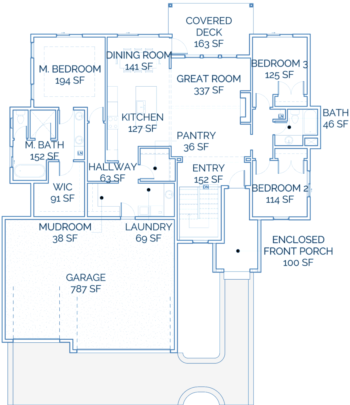
First floor NTS
