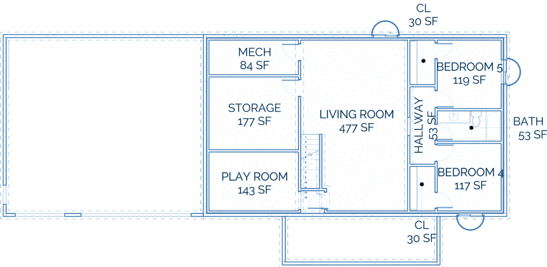
Basement NTS
